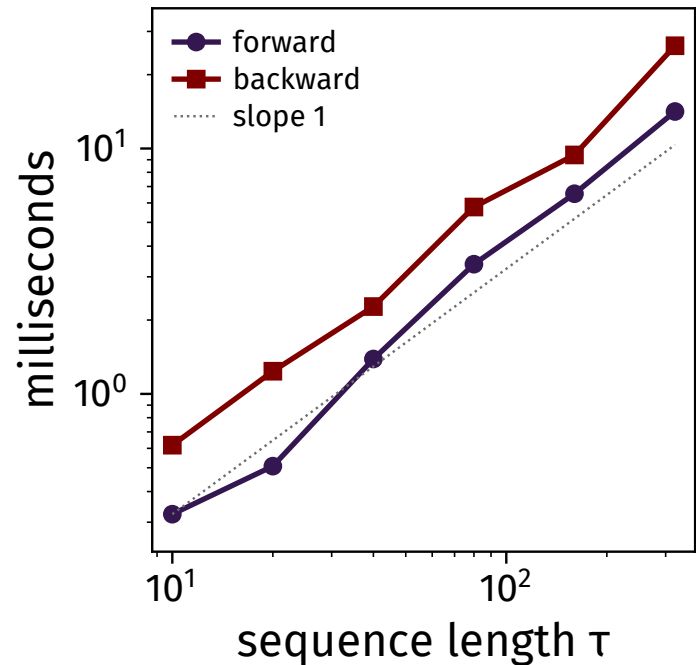
(a) time of one pass, O(\tau)
