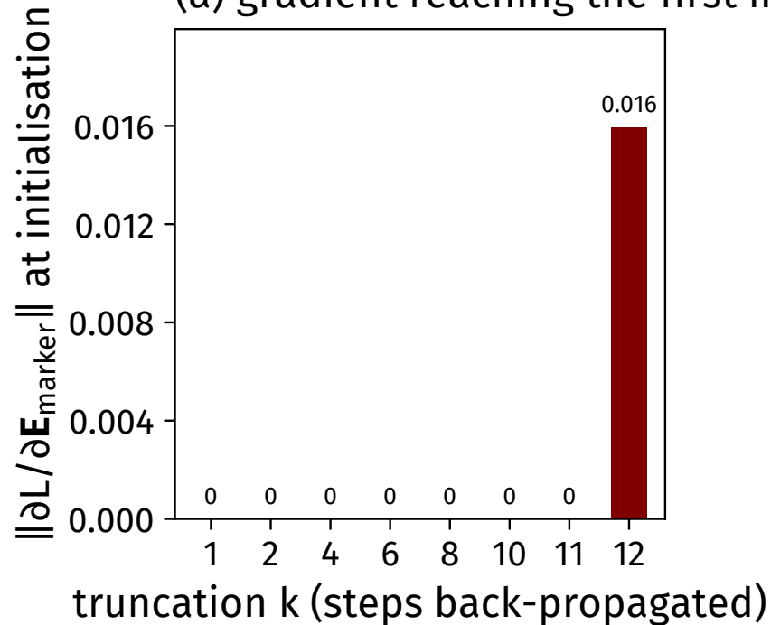
(a) gradient reaching the first input, \tau = 12
