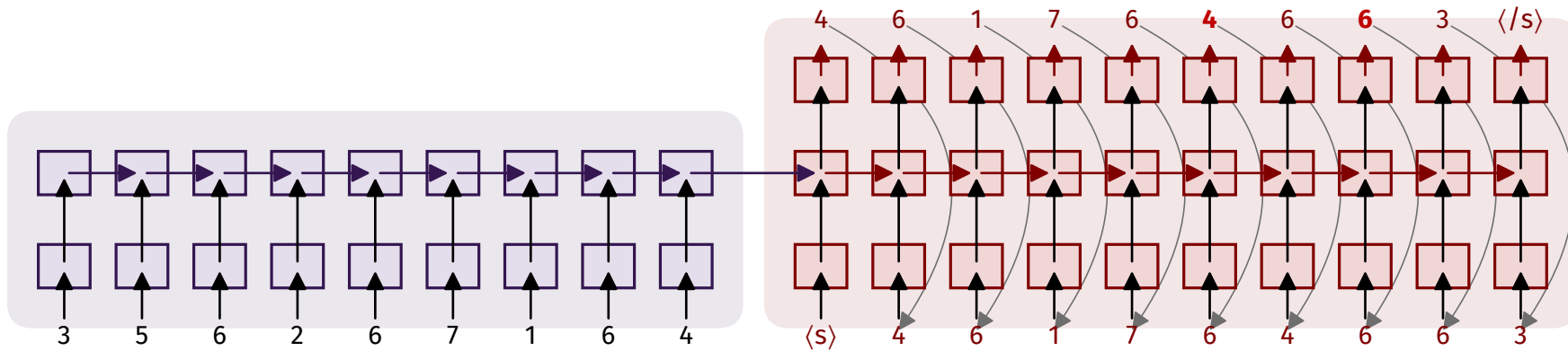
(a) inference: each input is the model's previous output; the bold red token is where it goes wrong
