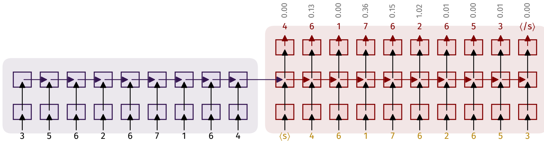
(b) training with teacher forcing: gold inputs (amber); the losses -\log p(\text{gold}) above average to 0.168
