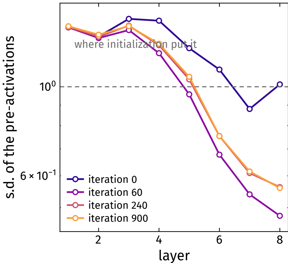
(a) the statistics drift as training proceeds
