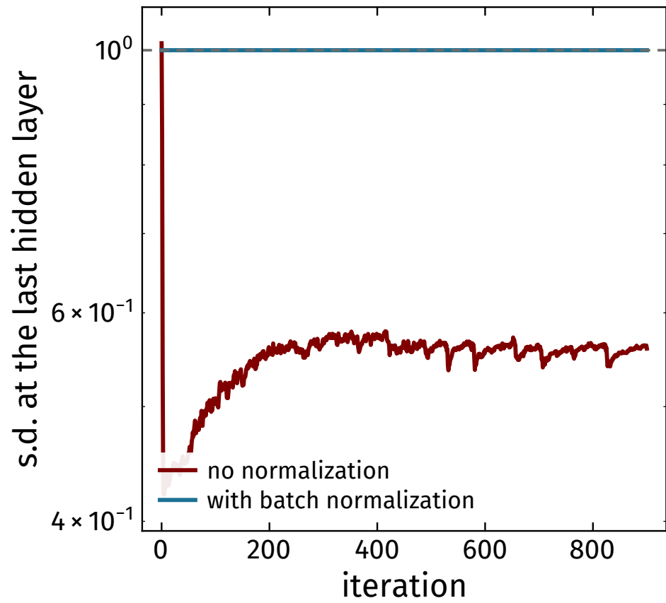
(b) a normalizer holds it in place
