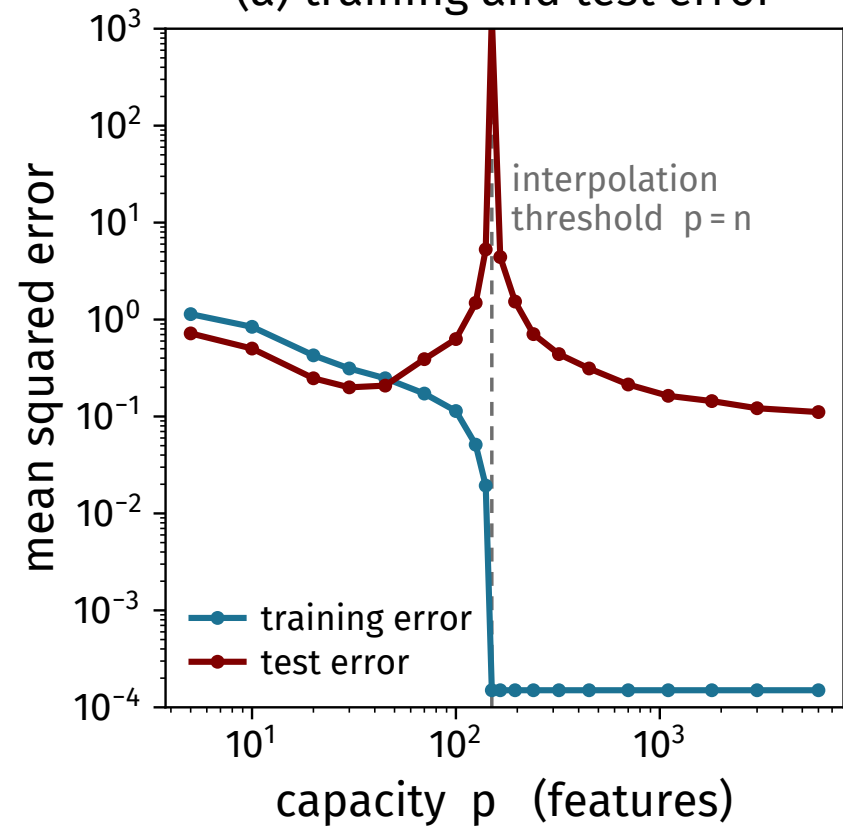
(a) training and test error
