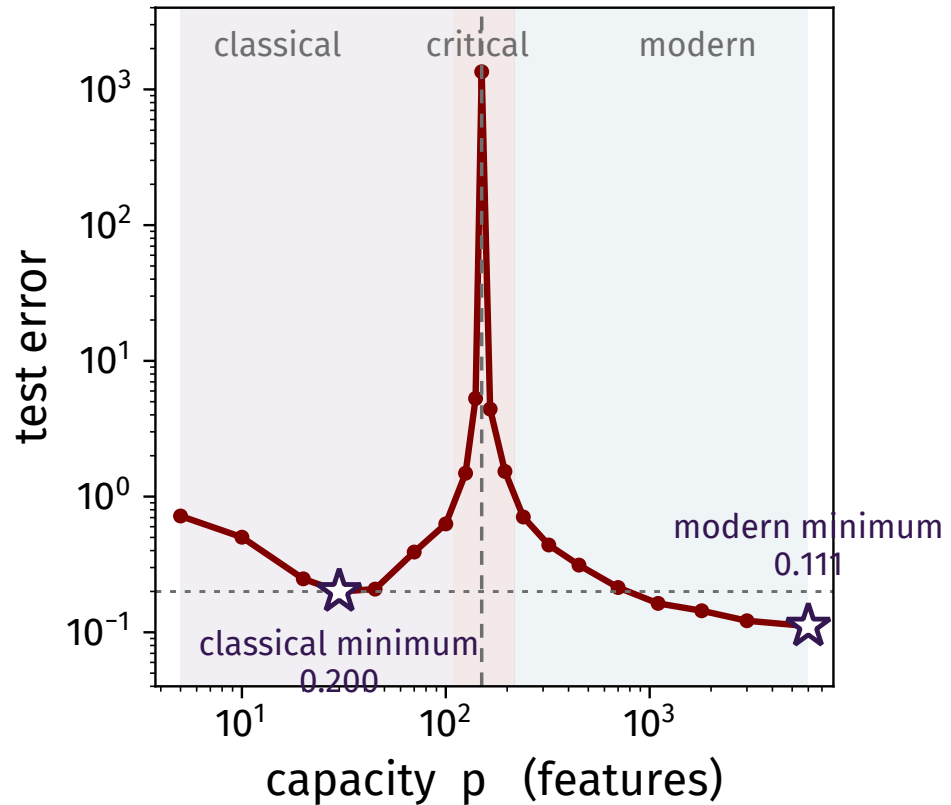
(b) three regimes, not two
