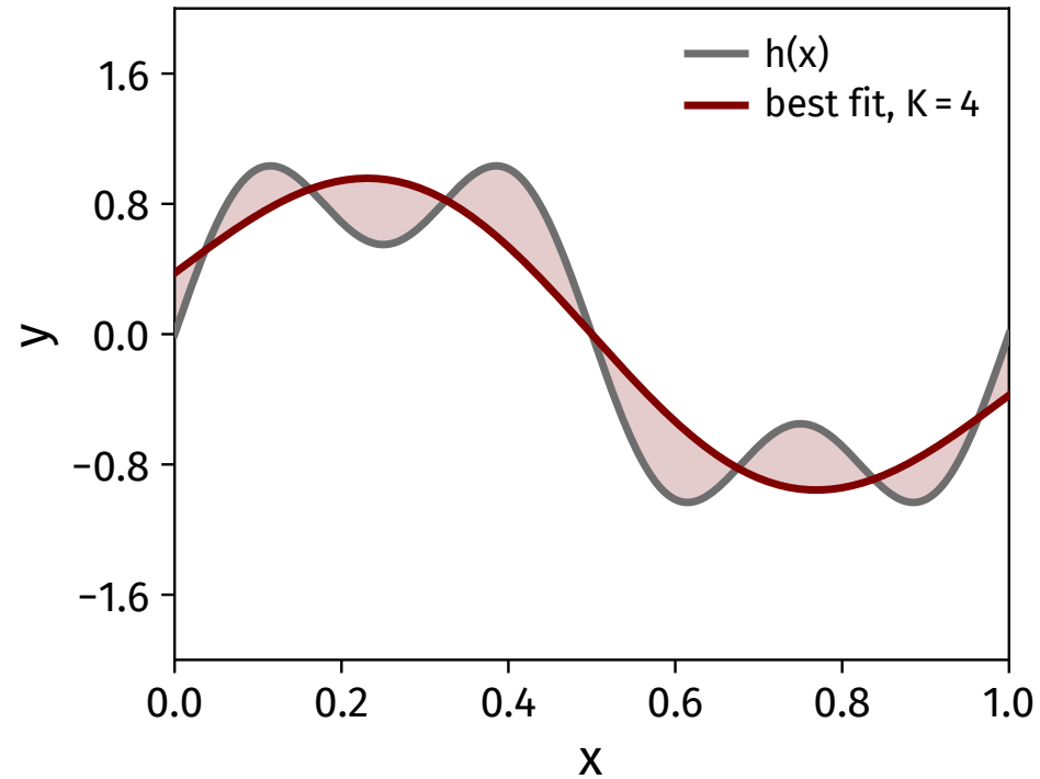
(b) bias: the best fit still misses
