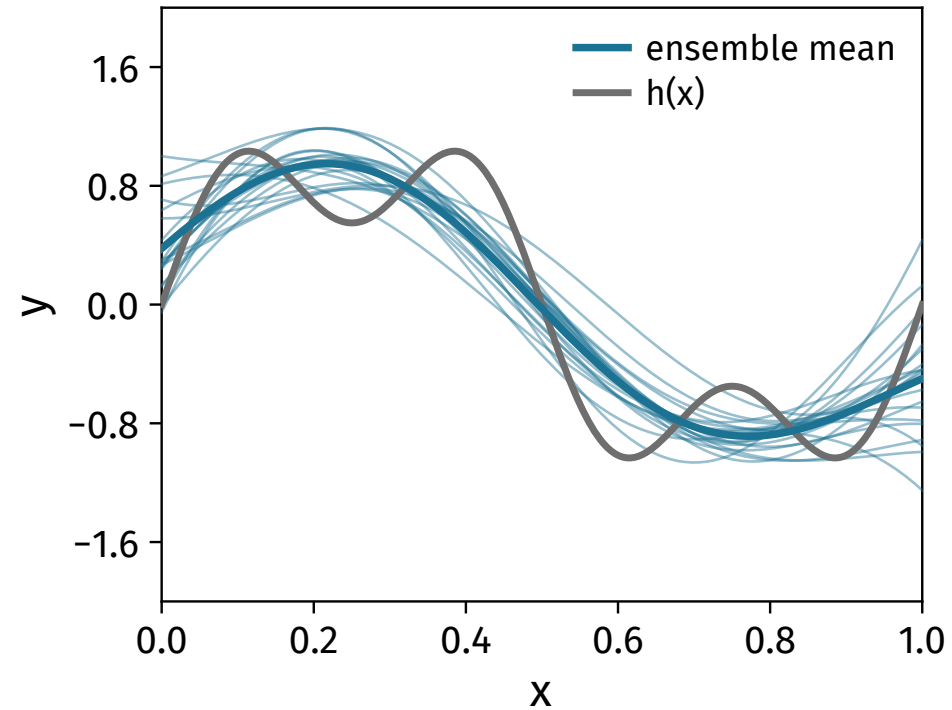
(c) variance: the fit moves with the sample
