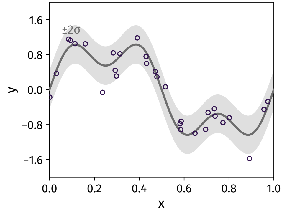
(a) noise: floor \sigma^2
