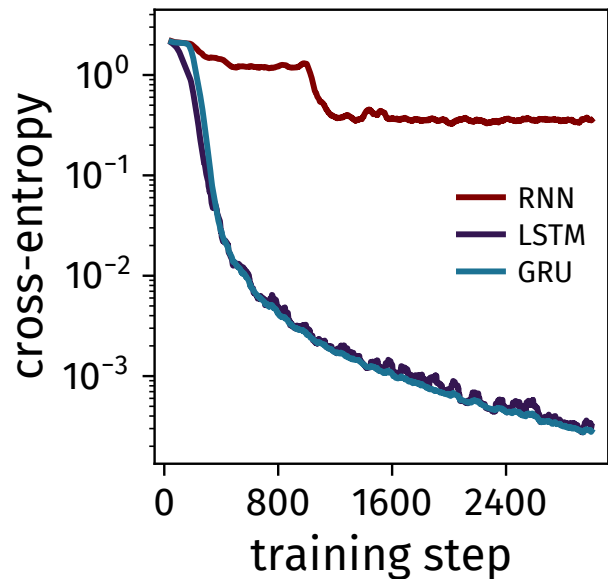
(a) training loss
