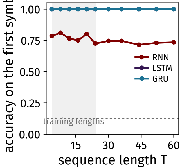
(b) recall by length
