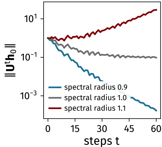
(a) the power method, three radii
