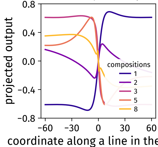
(b) a linear--tanh layer composed t times
