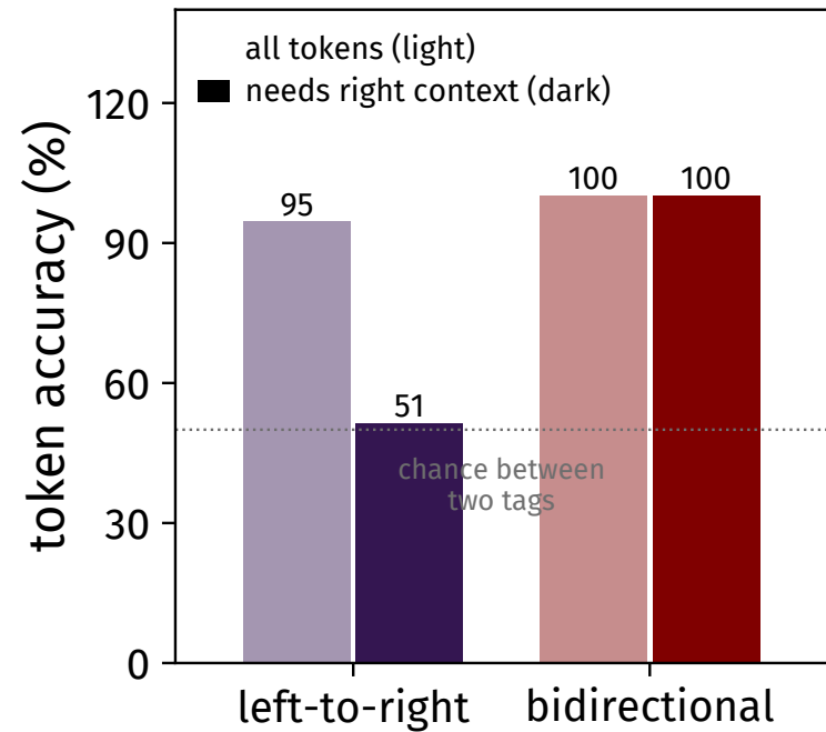
(a) accuracy on held-out sentences
