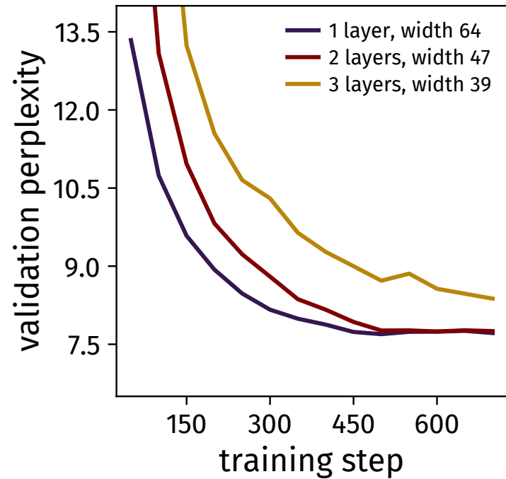
(a) matched parameters, \approx 38k
