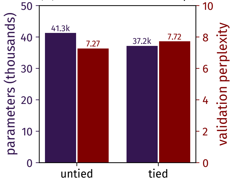
(b) the character model, |V| = 64 , d = 64
