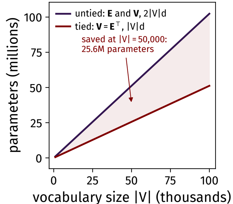
(a) embedding + output parameters, d = 512
