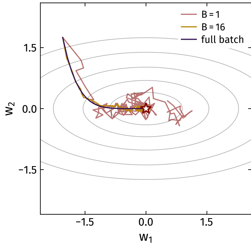
(a) trajectories, per iteration
