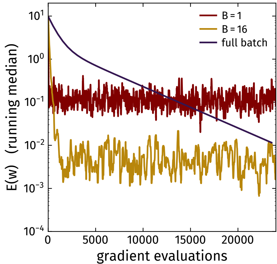
(b) the same runs, per unit of work
