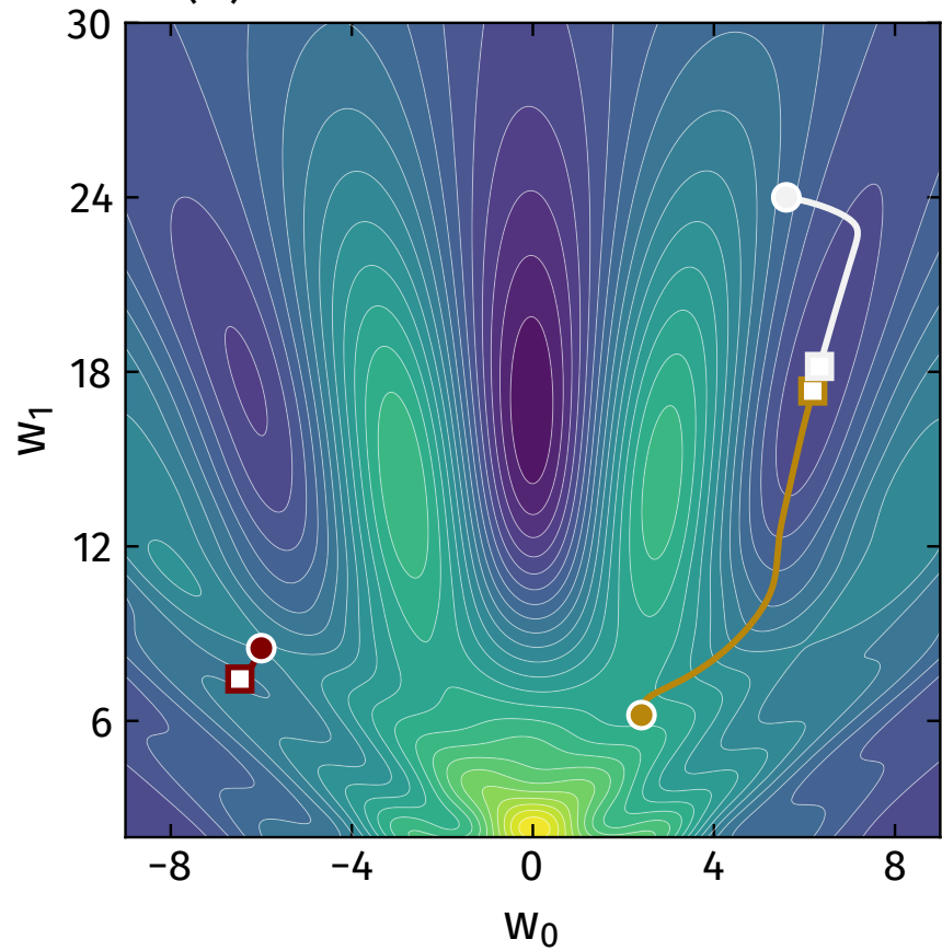
(b) the start decides the finish
