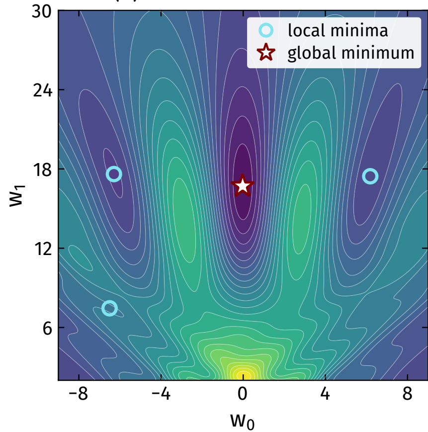
(a) the loss is not convex
