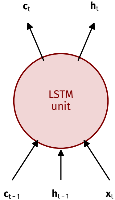
(c) an LSTM unit
