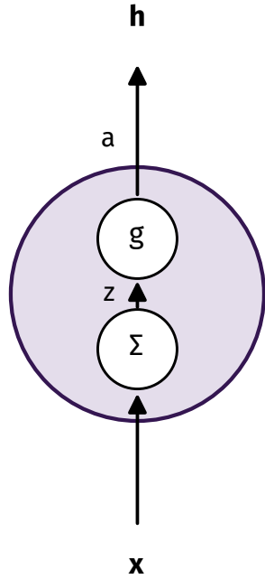
(a) a feedforward unit
