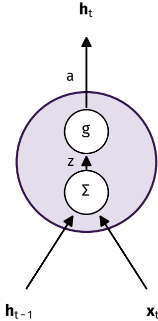
(b) a simple recurrent unit
