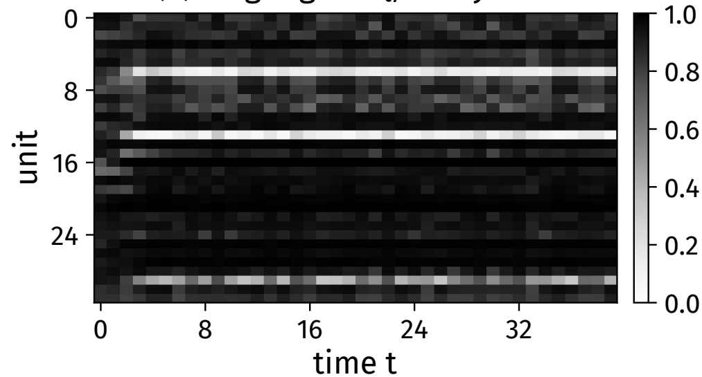
(a) forget gate \mathbf{f}_t , every unit
