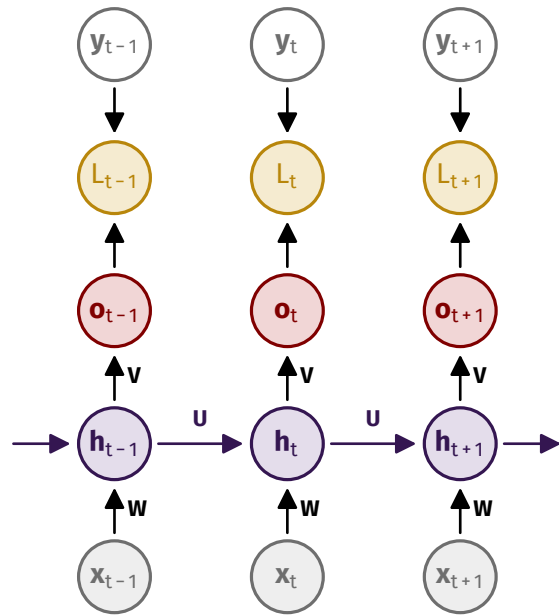
(a) hidden-to-hidden recurrence
