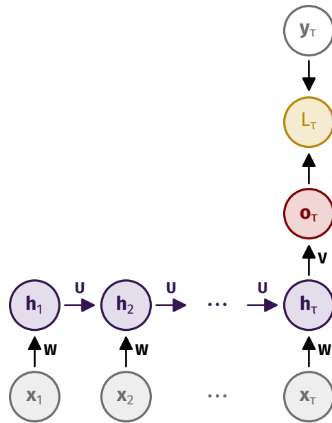
(c) a single output at the end
