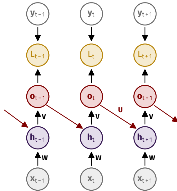
(b) recurrence from the output
