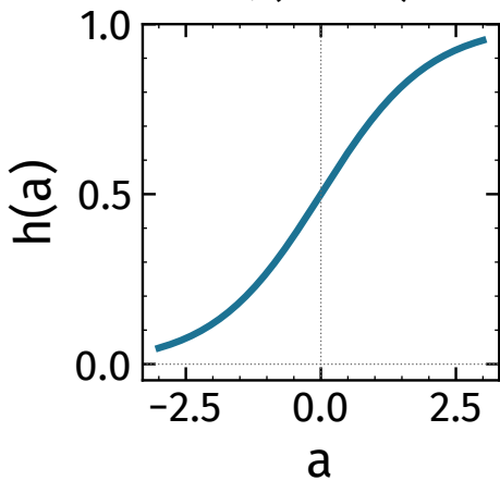
logistic sigmoid 1/(1 + e^{-a})
