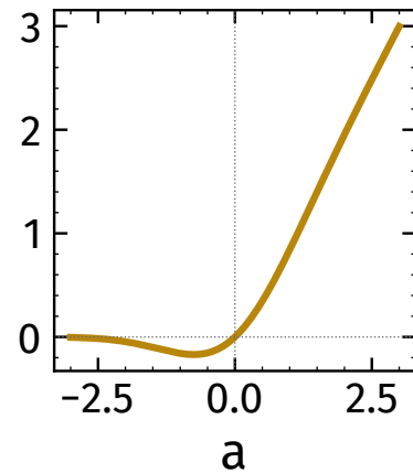
GELU a\Phi(a)
