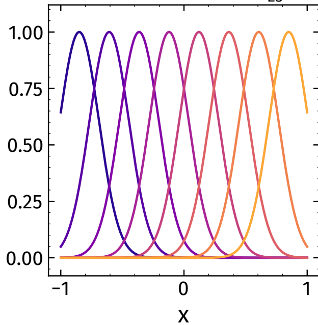
(b) Gaussian: \exp(-\frac{(x - \mu_j)^2}{2s^2})
