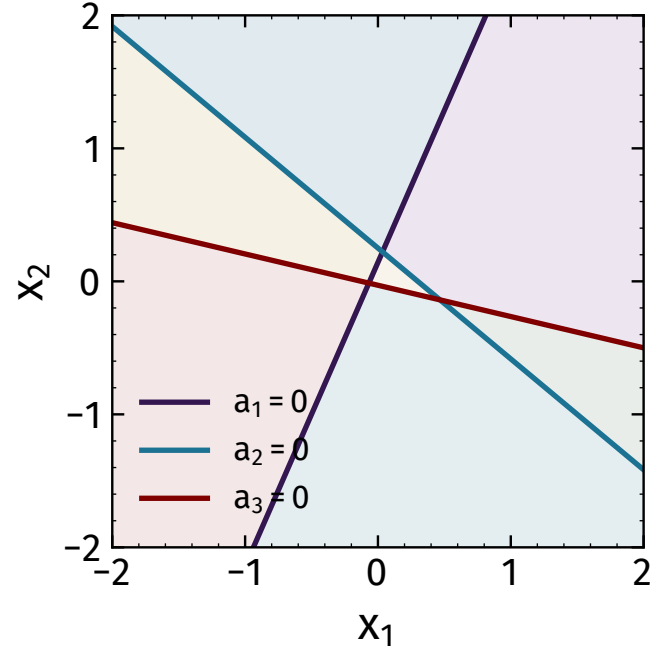
(a) M = 3 hinges cut the plane into convex regions
