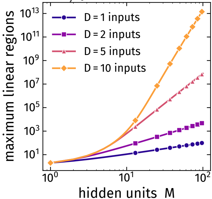
(a) \sum_{j=0}^D \binom{M}{j} (Zaslavsky, 1975)
