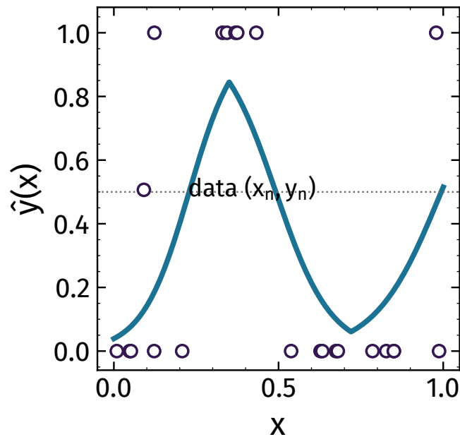
(b) \hat{y} = \sigma(a) : a probability
