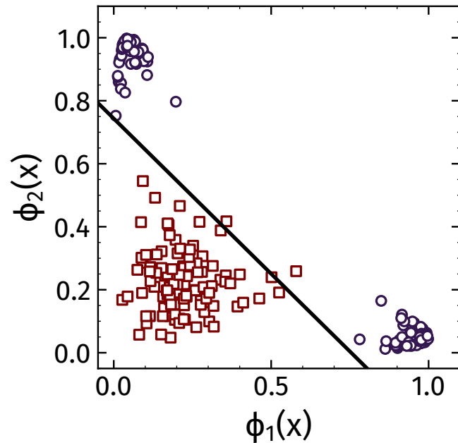
(b) fixed features: linearly separable
