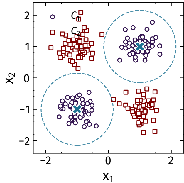
(a) input space: no straight line works
