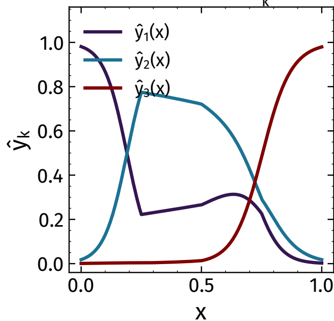
(b) after softmax: \sum_k \hat{y}_k = 1
