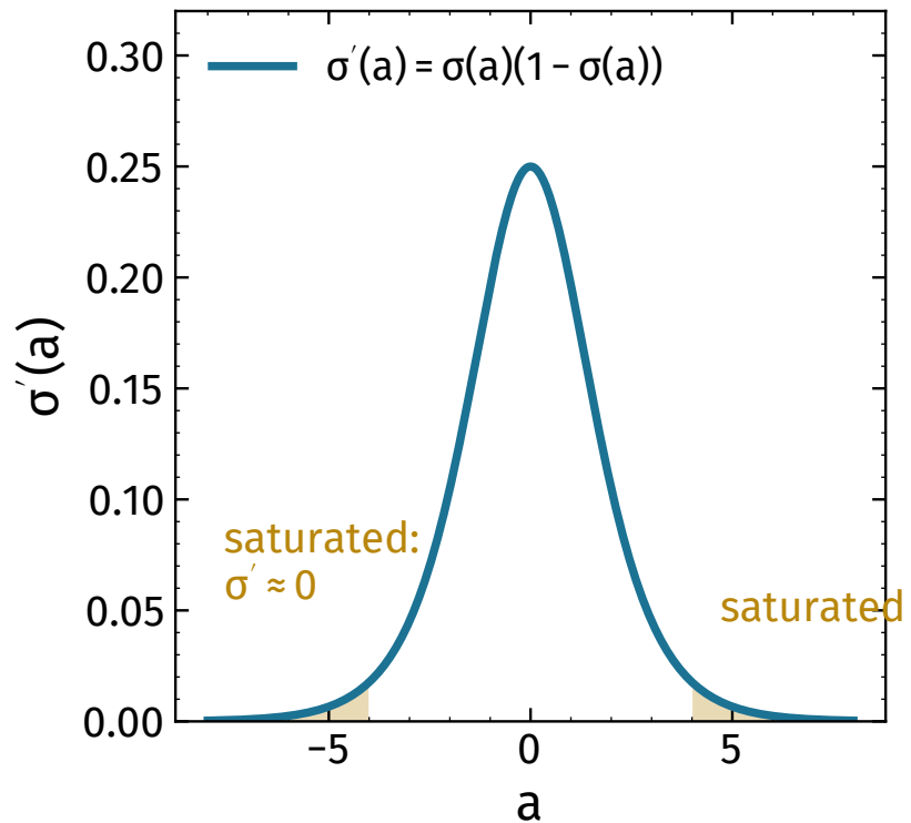
(b) the gradient dies in the tails
