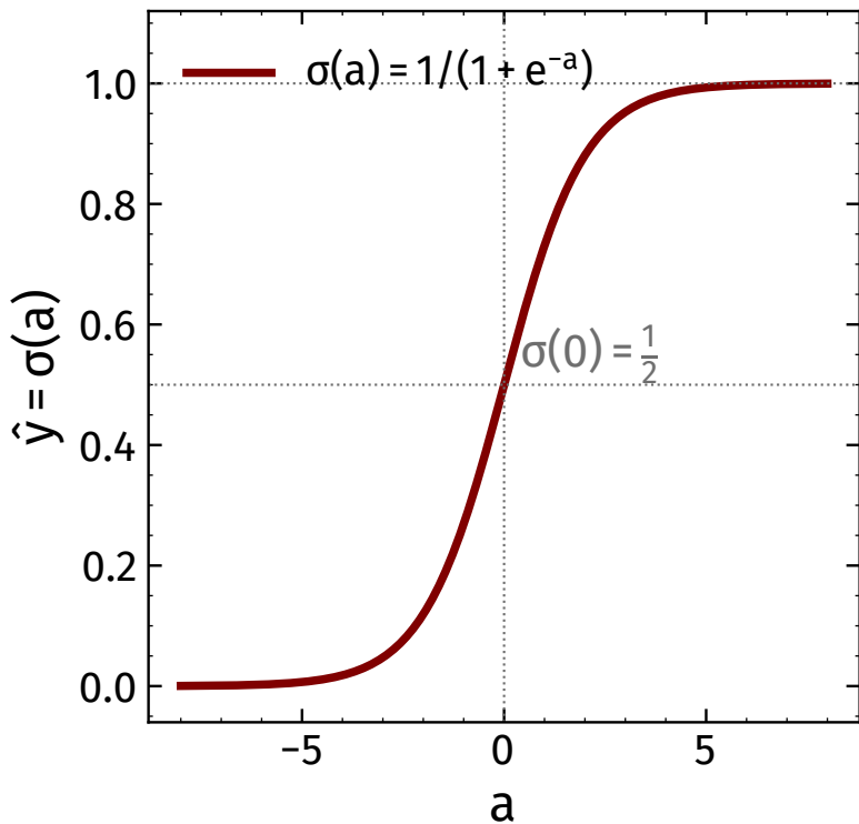
(a) maps \mathbb{R} onto (0,1)
