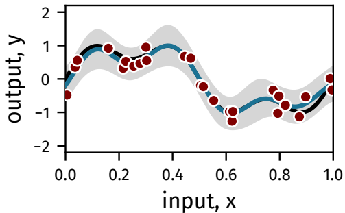
(e) predictive mean, \pm 2 s.d.
