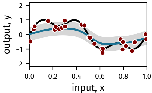
(f) predictive mean, \pm 2 s.d.
