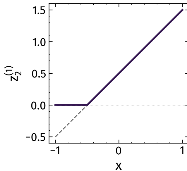
(b) z_2^{(1)} = h(x + 0.5)
