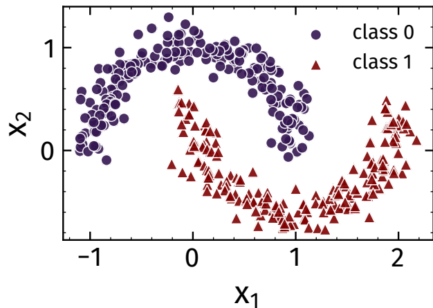
(a) input space: not linearly separable
