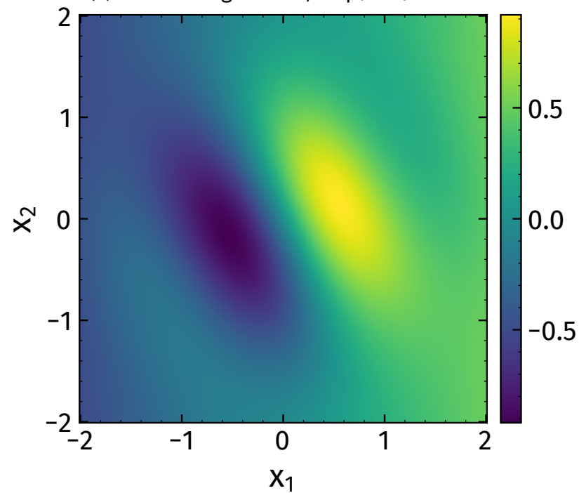
(c) K=220 ridge terms, \sup |f - \hat{f}| = 0.023
