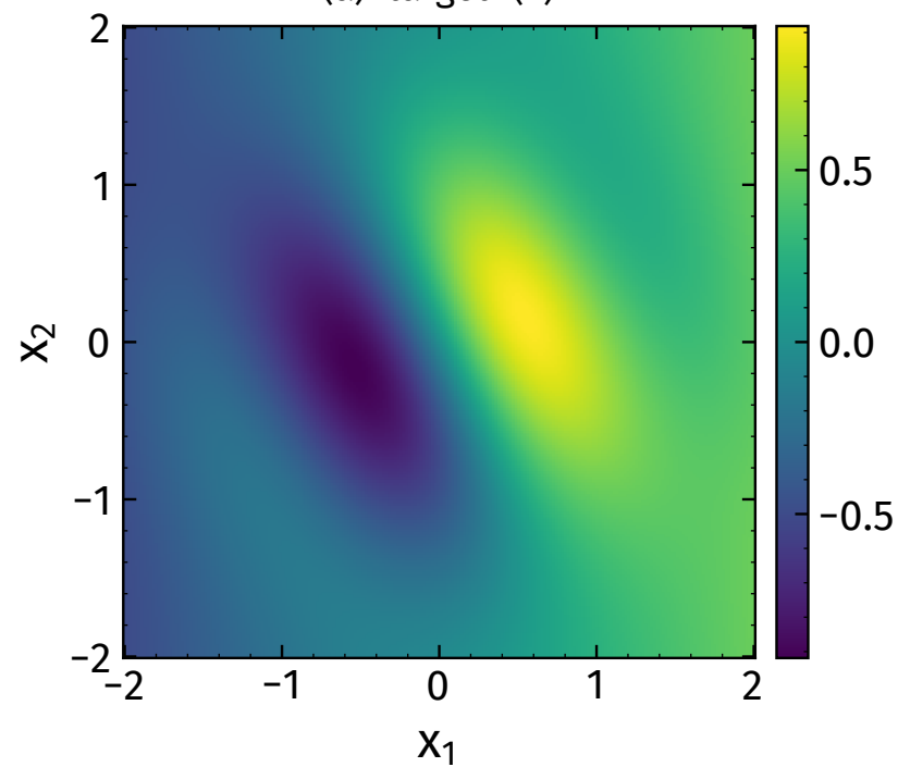
(a) target f(\mathbf{x})
