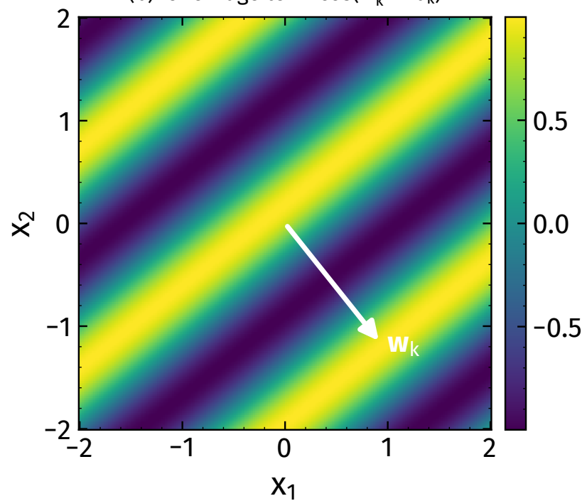
(b) one ridge term \cos(\mathbf{w}_k^T \mathbf{x} + b_k)
