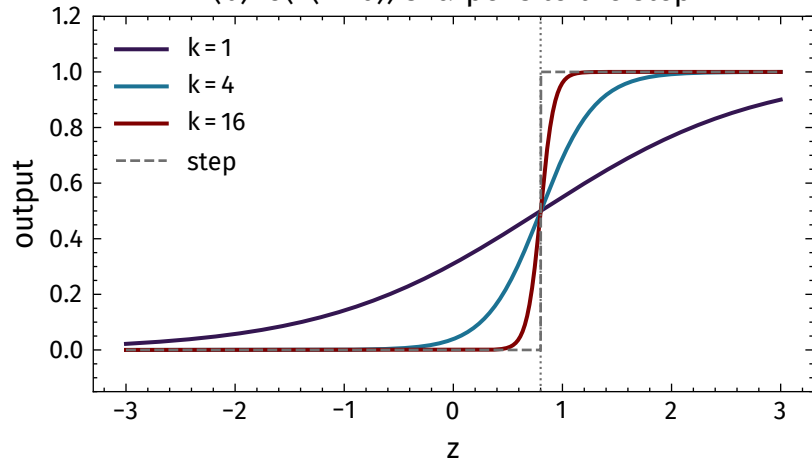
(b) \sigma(k(z - \theta)) sharpens to the step
