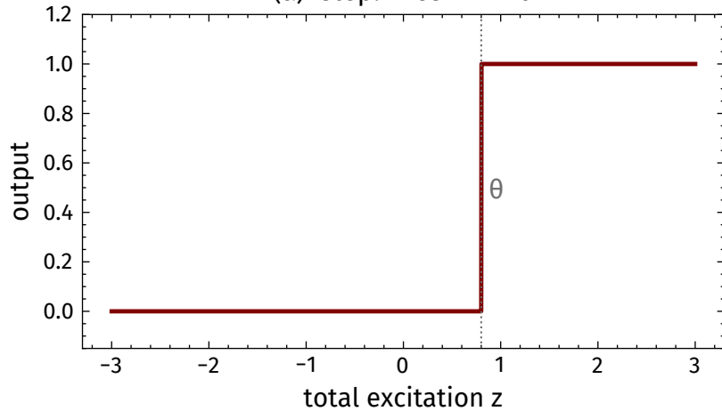
(a) step: fires iff z \geq \theta
