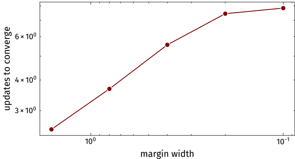
(b) narrow margins cost more updates
