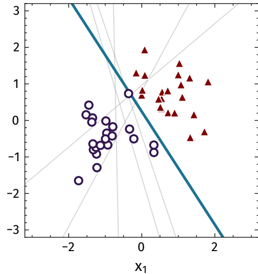
converged: 5 updates
