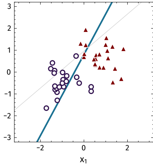
after 1 update
