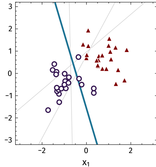
after 3 updates
