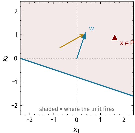
(b) after: w' = w + x
