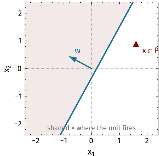
(a) before: w \cdot x < 0
