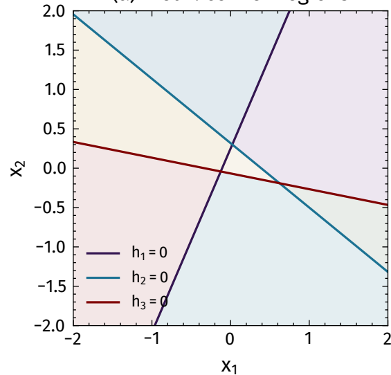
(a) net 1: convex regions
