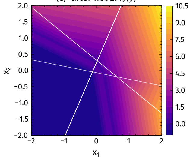
(c) after net 2: f_2(y)
