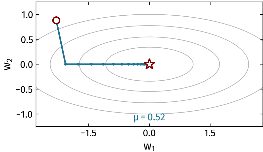
(b) Nesterov momentum
