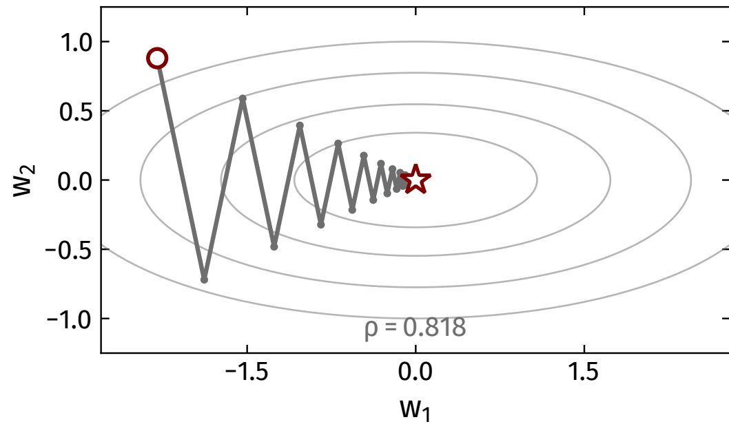
(a) gradient descent
