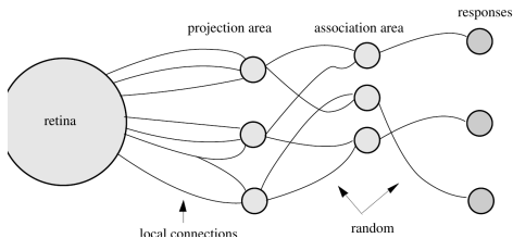
Rojas (1996), Fig. 3.1: the classical perceptron [after Rosenblatt 1958].
