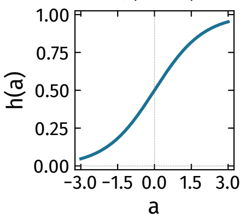
logistic sigmoid 1/(1 + e^{-a})
