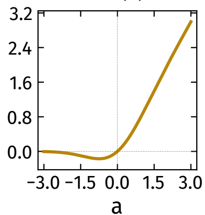
GELU a\Phi(a)
