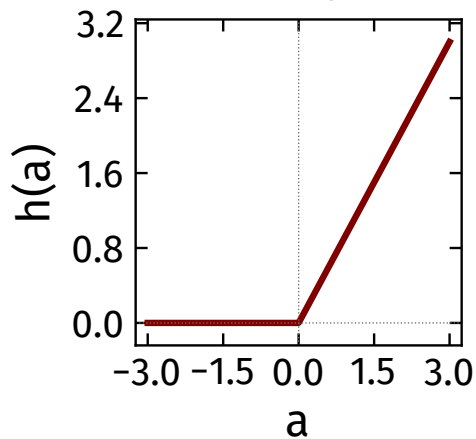
ReLU \max(0, a)
