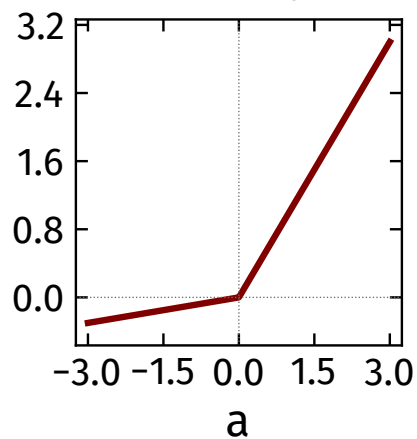
leaky ReLU \max(0.1a, a)
