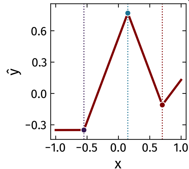
(f) one joint per unit, at x = -w_{j0}^{(1)} / w_{j1}^{(1)}
