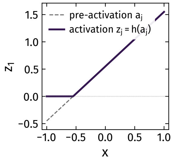
(a) z_1 = h(1x + 0.55)
