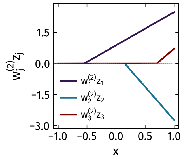
(d) each unit scaled by its output weight
