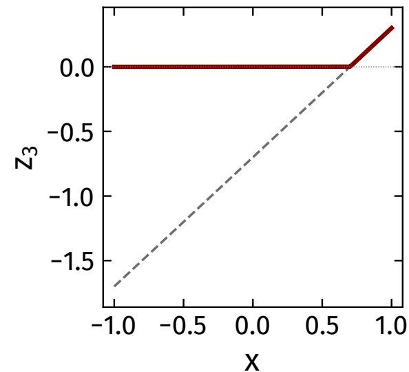
(c) z_3 = h(1x - 0.70)
