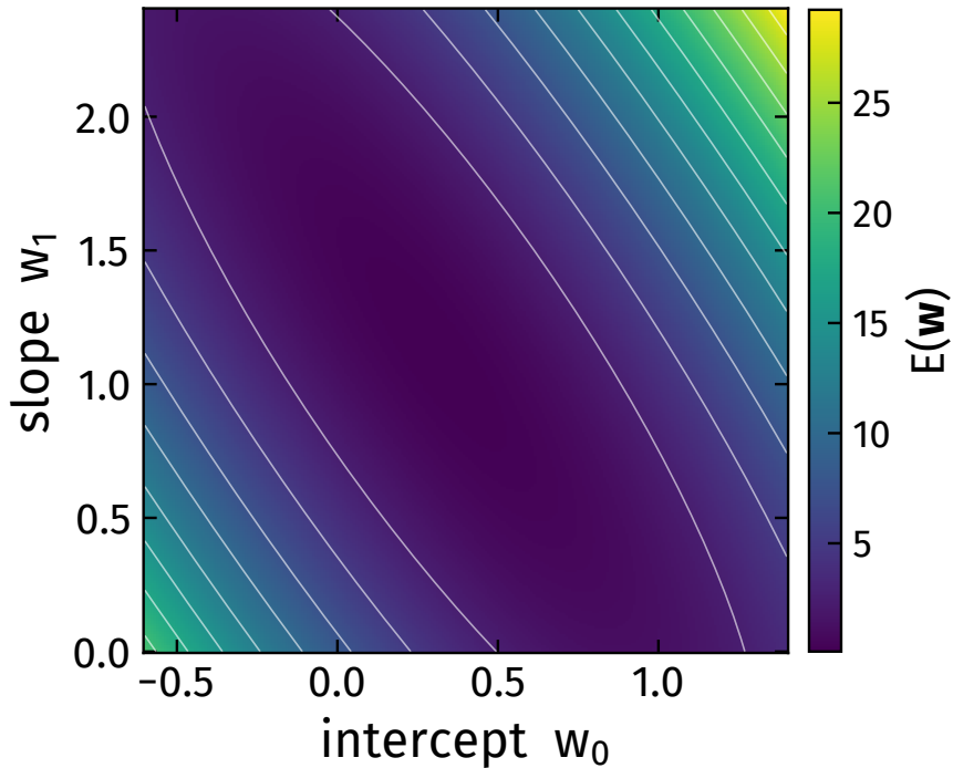
(a) the error surface E(\mathbf{w})
