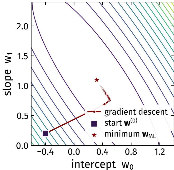
(b) one convex bowl, one minimum
