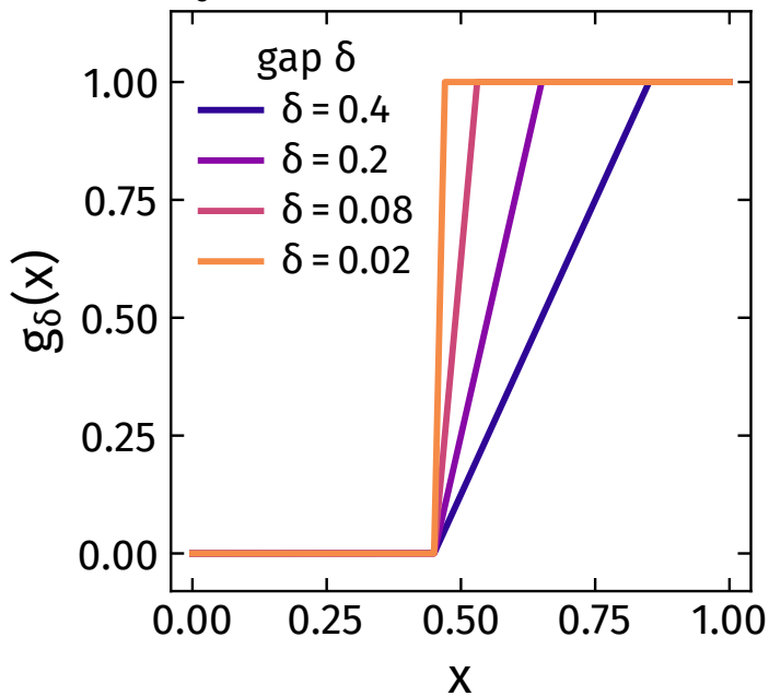
(a) \frac{1}{\delta}[h(x-a) - h(x-a-\delta)] \rightarrow \mathbb{1}[x > a]
