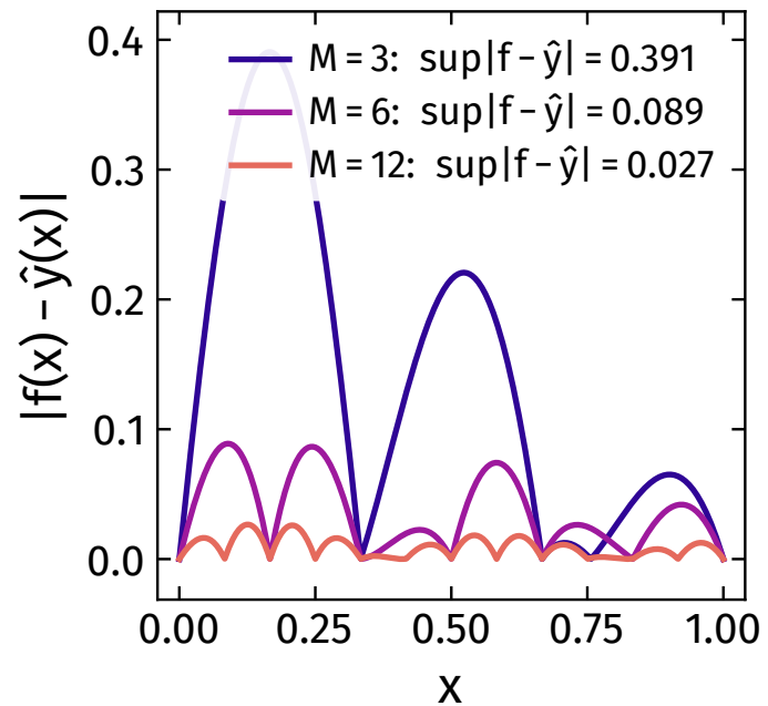
(c) \text{mesh} < \delta \Rightarrow \sup|f - \hat{y}| \leq \varepsilon
