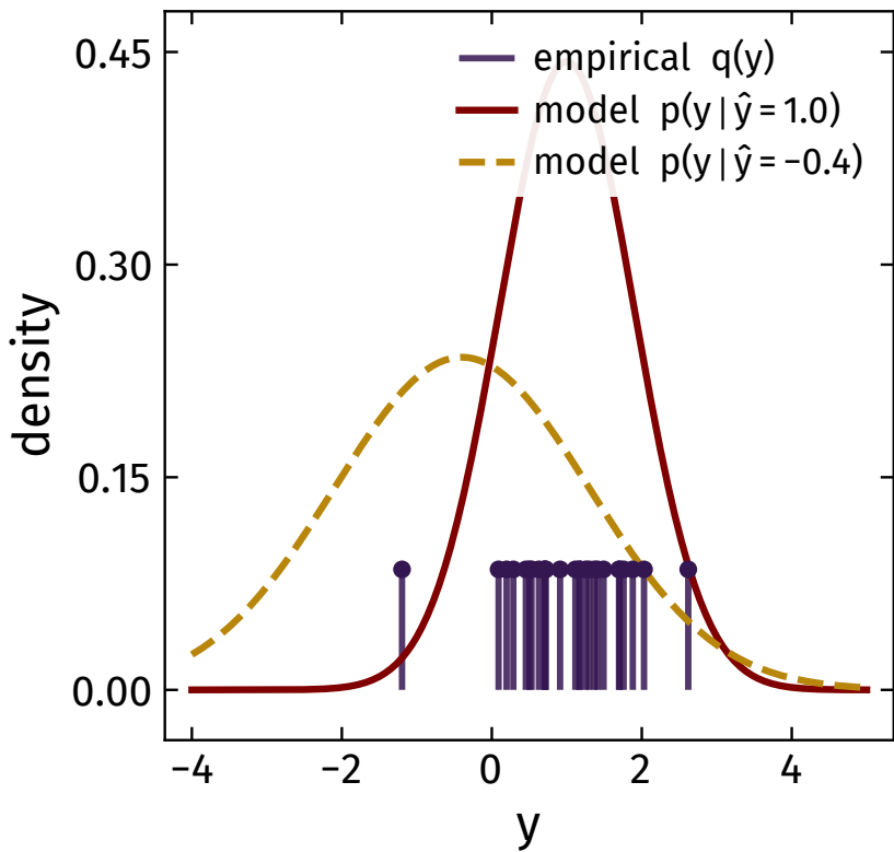
(a) fit the model to the empirical distribution
