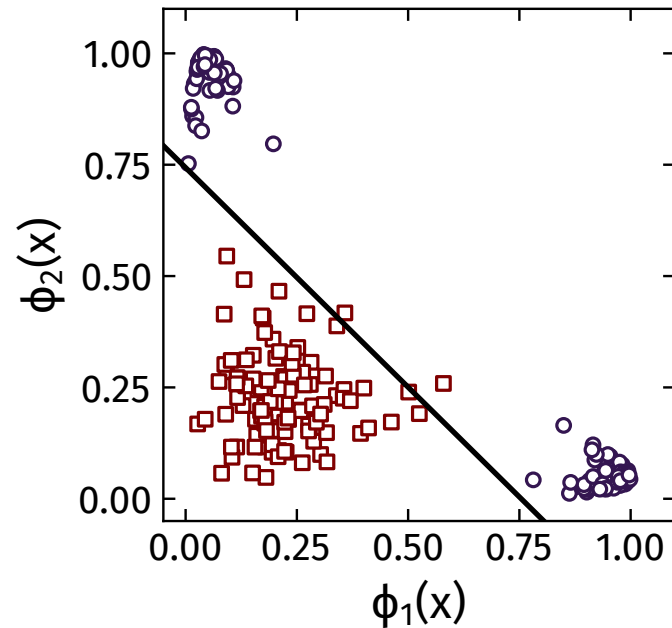
(b) fixed features: linearly separable
