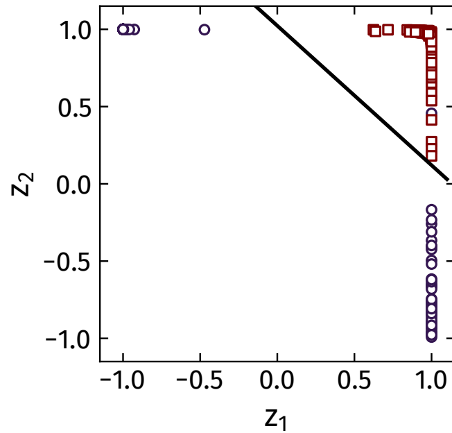
(c) learned features (tanh): also linear
