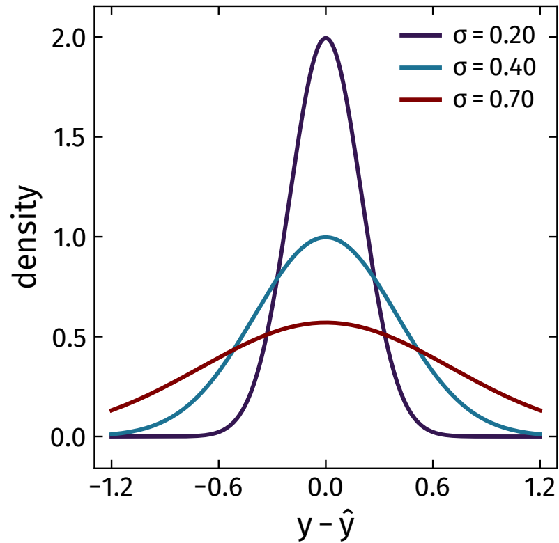
(b) -\ln p \propto (y - \hat{y})^2 : squared error
