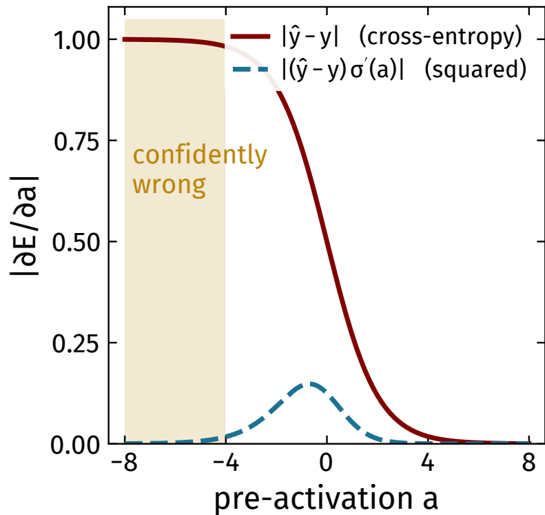
(b) squared error stops learning; cross-entropy does not
