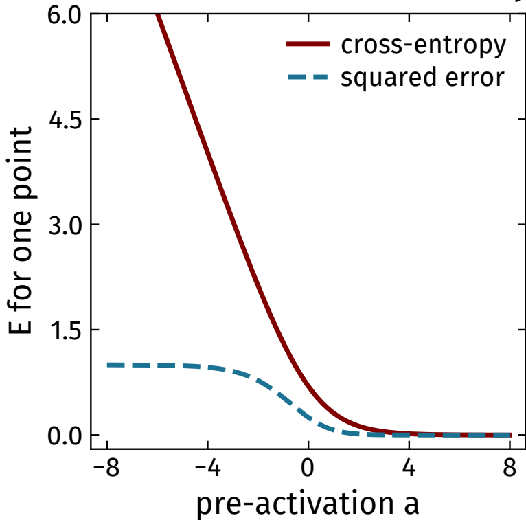
(a) the error when the true label is y = 1
