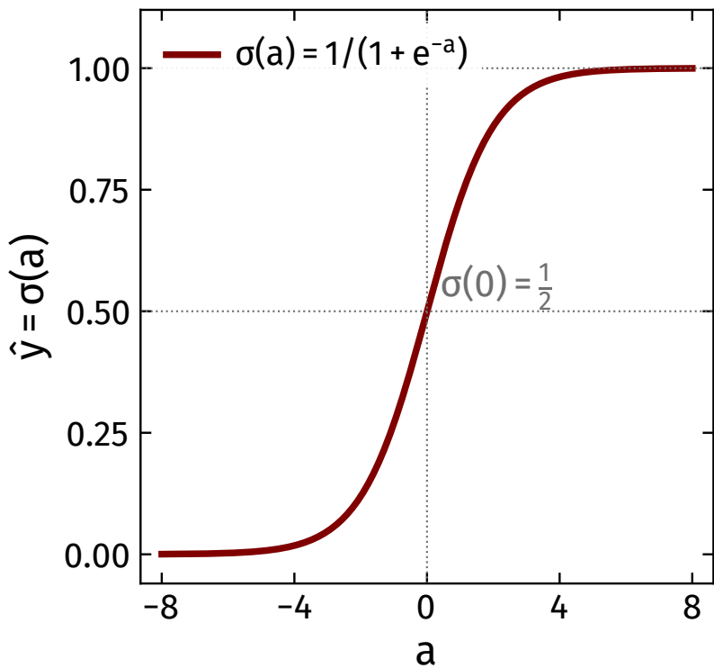
(a) maps \mathbb{R} onto (0, 1)
