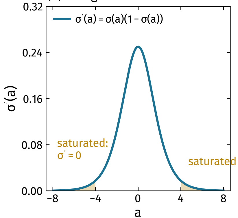
(b) the gradient dies in the tails
