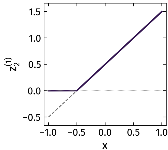
(b) z_2^{(1)} = h(x + 0.5)
