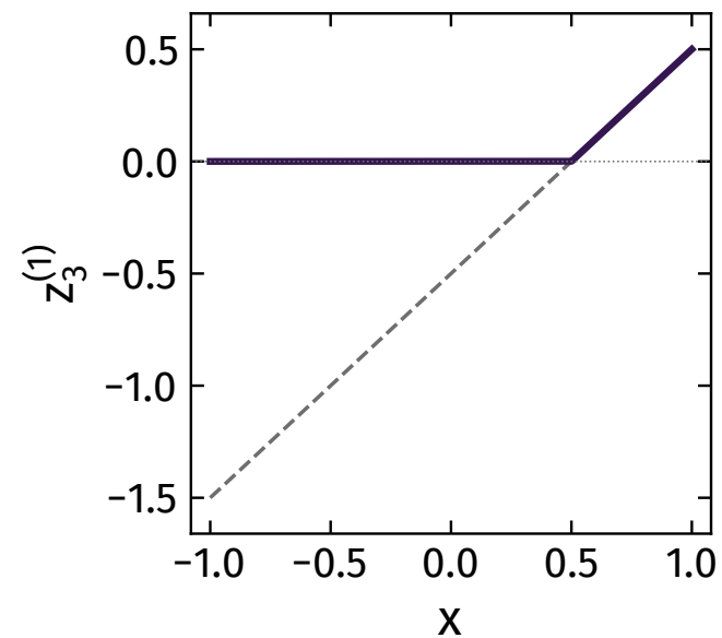
(c) z_3^{(1)} = h(x - 0.5)
