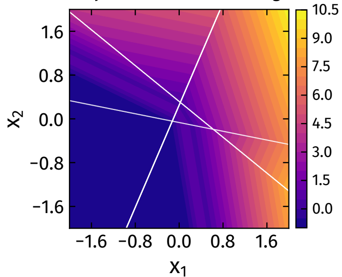
(c) layer 2 subdivides each region
