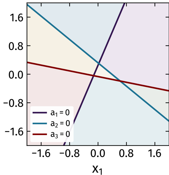
(a) layer 1: convex regions
