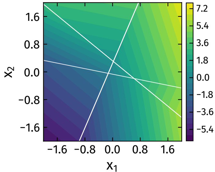
(b) its output: planar per region
