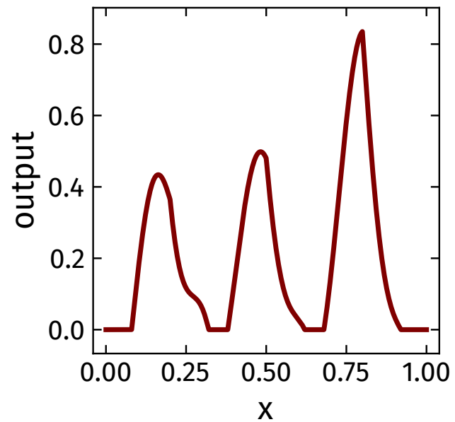
(c) level 3: the motif, modulated
