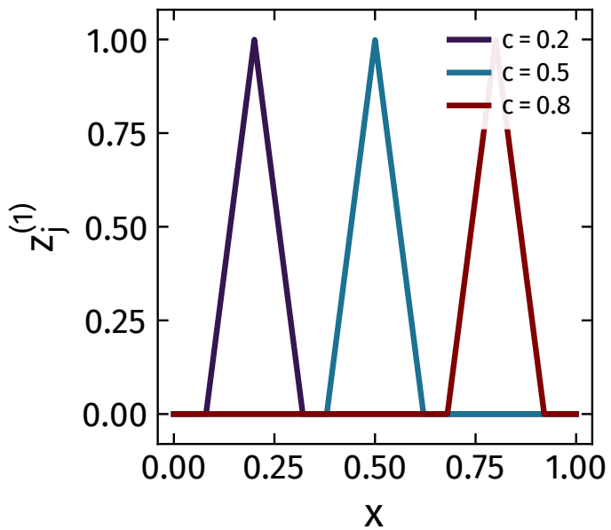
(a) level 1: parts, h(1 - |x - c|/w)
