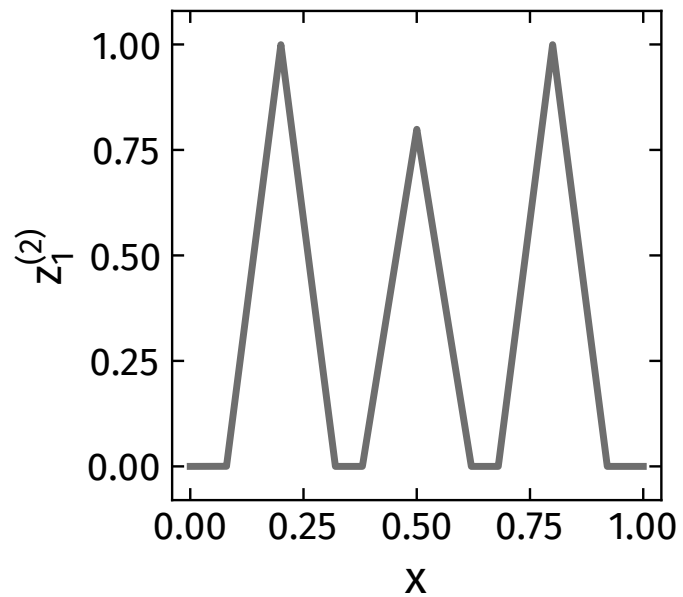
(b) level 2: one motif from three parts
