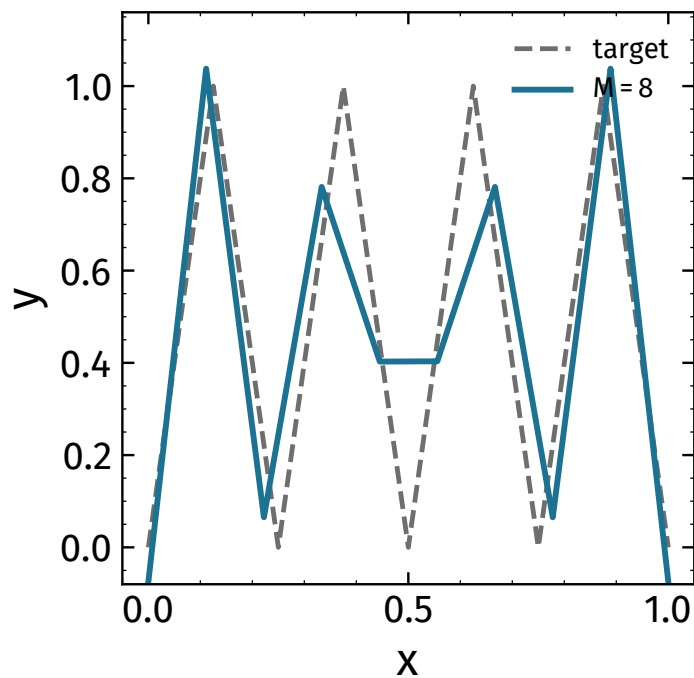
(b) shallow, M=8 : \sup|f-\hat{y}| = 0.403
