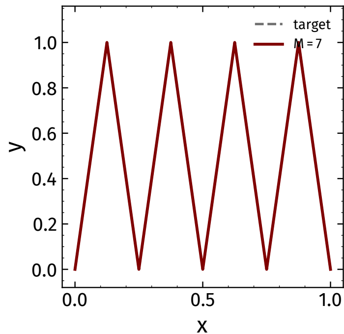
(c) shallow, M=7 : \sup|f-\hat{y}| = 0.000
