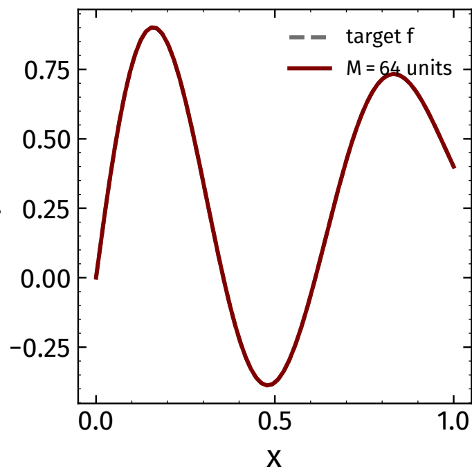
(c) M = 64 : \sup|f - \hat{y}| = 0.0015
