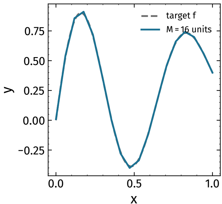
(b) M = 16 : \sup|f - \hat{y}| = 0.0224
