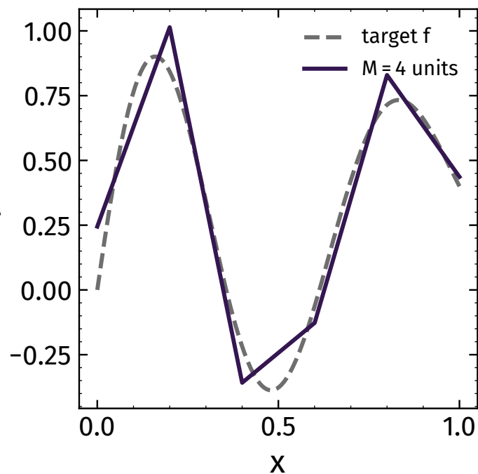
(a) M = 4 : \sup|f - \hat{y}| = 0.2446
